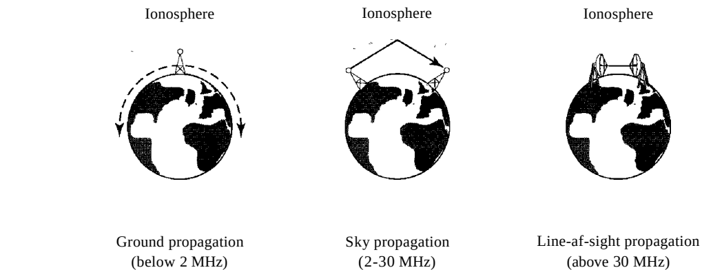
Figure 7.18 Propagation methods
