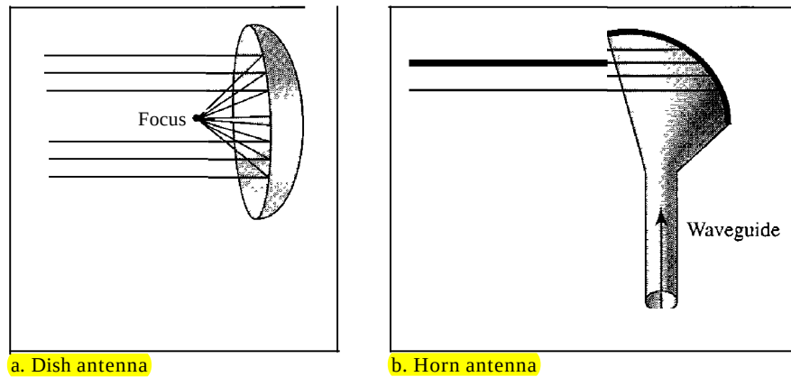
Figure 7.21 Unidirectional antennas
